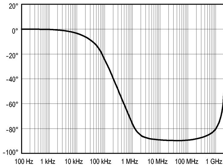
Figure 6: Typical Phase versus Frequency
