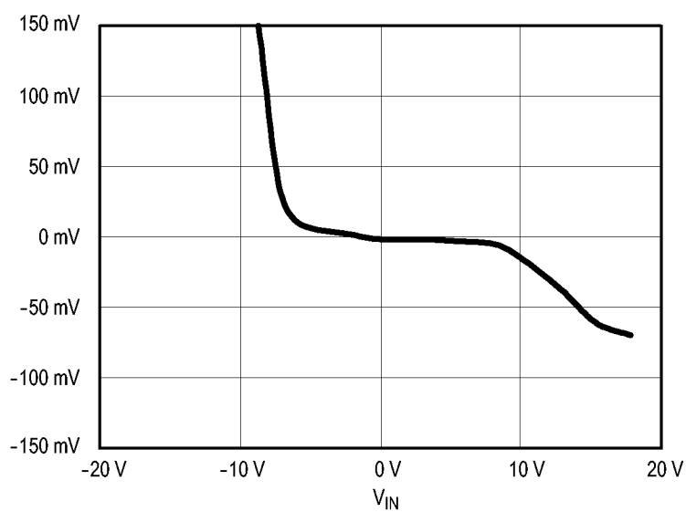
Figure 4: Typical Linearity Error versus V_{IN}
